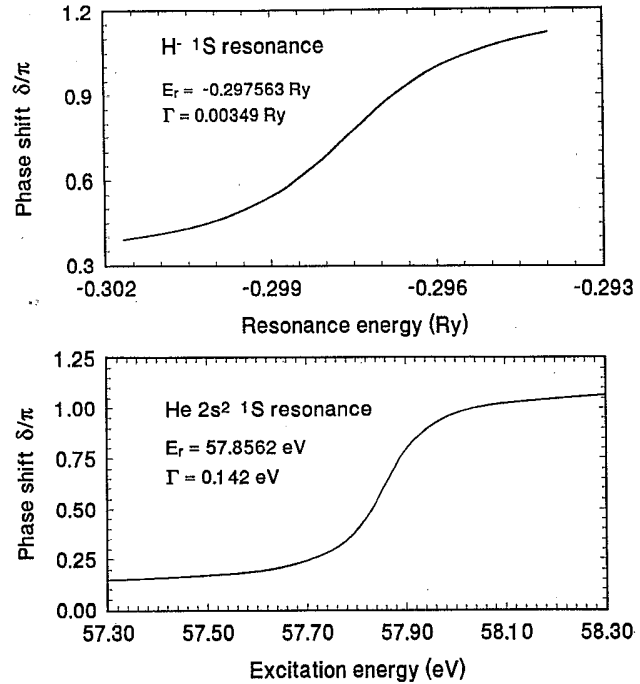
FIG. 3. The energy variation of the phase shifts for the lowest ^1S Feshbach resonance below the n=2 threshold for H^- and He.
