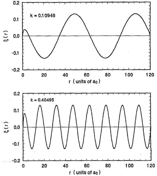
FIG. 1. The calculated one-particle functions \xi(r) representing the H^- 1ss configuration series at momenta k=0.10949 and 0.40495 .
