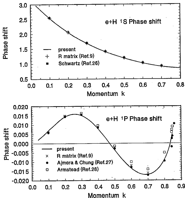
FIG. 2. The calculated S - and P -wave phase shifts for the electron-hydrogen scattering. The R -matrix results are taken from Ref. [9]. Other data shown are taken from Refs. [26], [27], and [28].
