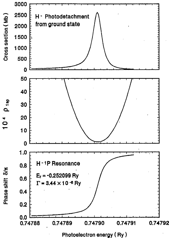
FIG. 6. The H^- photodetachment cross sections near the 1P Feshbach resonance below the n=2 threshold from the ground state. The calculated probability densities \rho_{1sp} due to the 1sp configuration series and the corresponding phase shifts are also plotted as functions of photoelectron energy for comparison.
