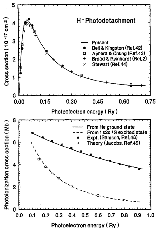
FIG. 4. The photoionization cross sections below the resonance structure for H^- and He. Comparisons are made with data taken from Refs. [42], [43], [2], [44], [49], and [48].
