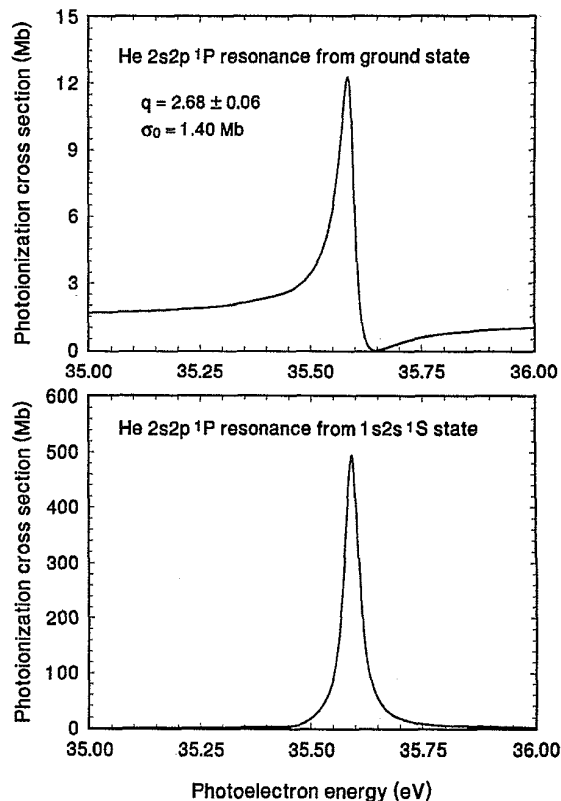
FIG. 5. The photoionization cross sections in the vicinity of 2s2p\ ^1P resonance from both the ground state and the 1s2s\ ^1S excited state of He.
